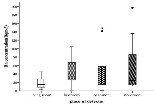
Figure 6. Radon concentration variations in different places of dwellings
